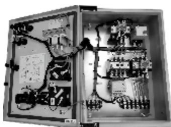
Fully Automatic Star Delta Starter with NHD Contactor, Electronic Timer & Electronic Over Current Relay with Ammeter & Voltmeter and MCB
